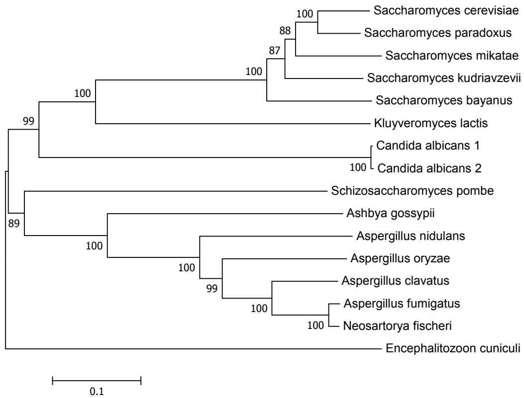
Fungi telomerase reverse transcriptase
